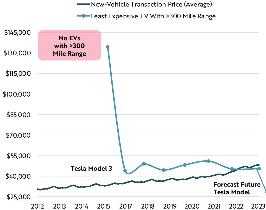
Transaction Price
